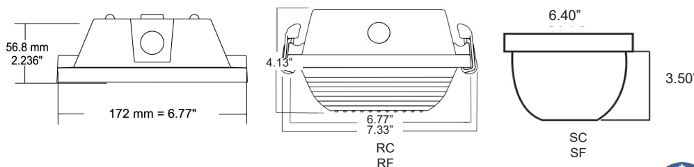
End View
