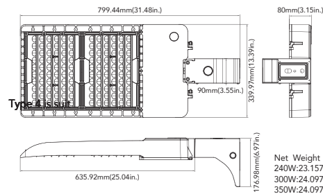
Pole Mount(240W&300W&350W)
