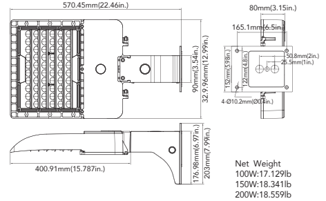
Wall Mount(100W/150W&200W)
