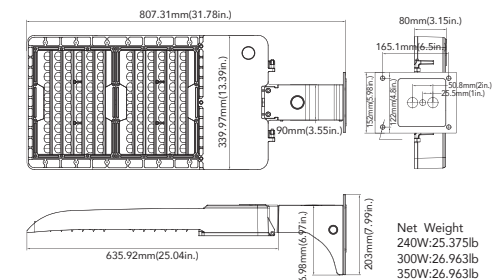
Wall Mount(240W&300W&350W)
