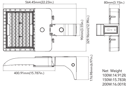
Pole Mount(100W/150W&200W)
