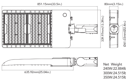
Slipfitter Mount(240W&300W&350W)
