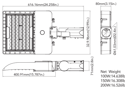
Slipfitter Mount(100W/150W&200W)
