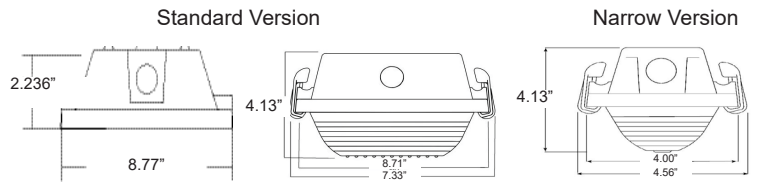
End View
