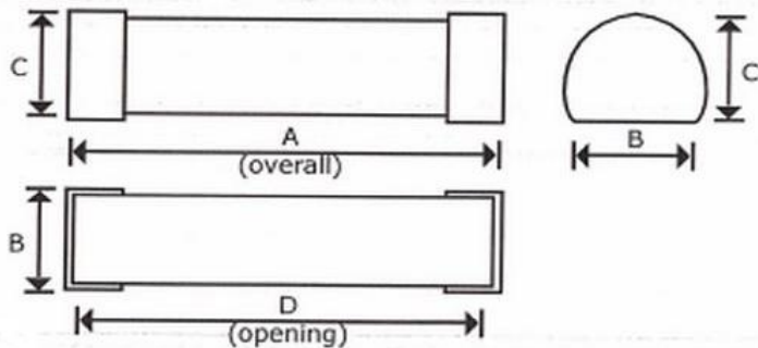
Standard End Cap (1 1/2" wide) - EC
