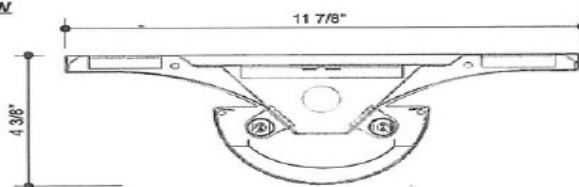
1X4 2 LAMP SHOWN. OPTIONAL RADIAL CROSS BAFFLE SHOWN
