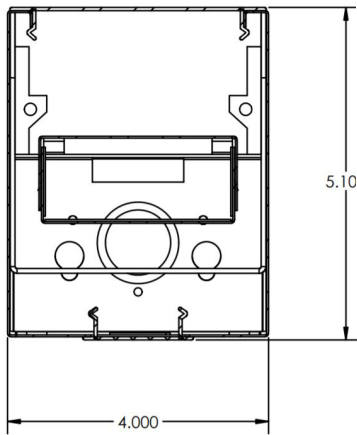
End View
